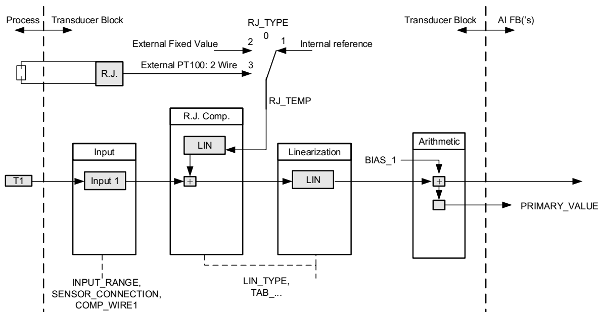
Figure 3.3 Transducer block structure
